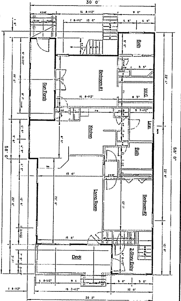
TYPICAL FLOOR SQUARE FOOTAGE FIRST FLOOR 1,469 S.F. (GROSS) DECK AREA 133 S.F. (GROSS) FIRST LEVEL FLOOR PLAN UNITS 1, 3, 5, 7, 9
